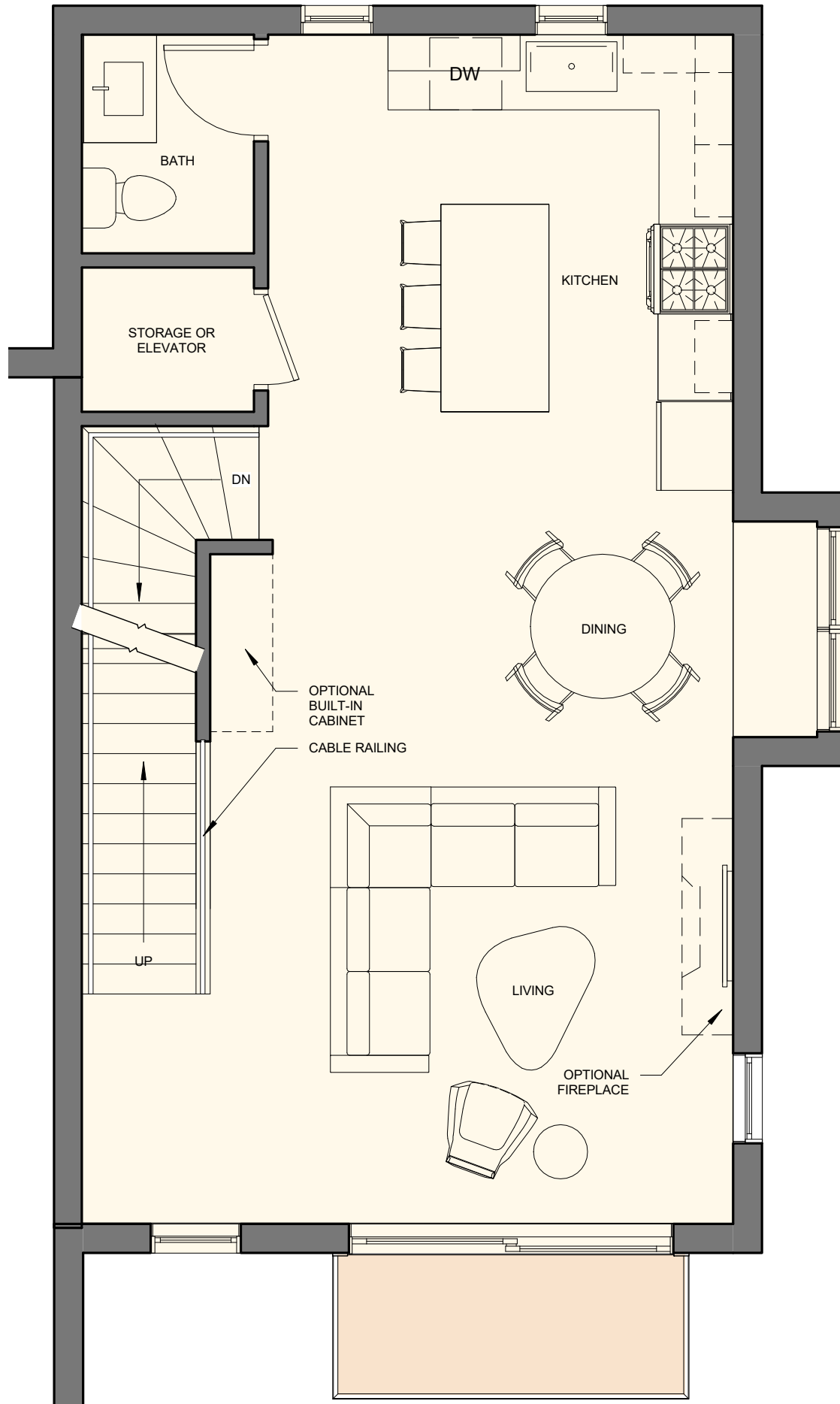
UNIT 1 SECOND FLOOR PLAN 1/4" = 1'
