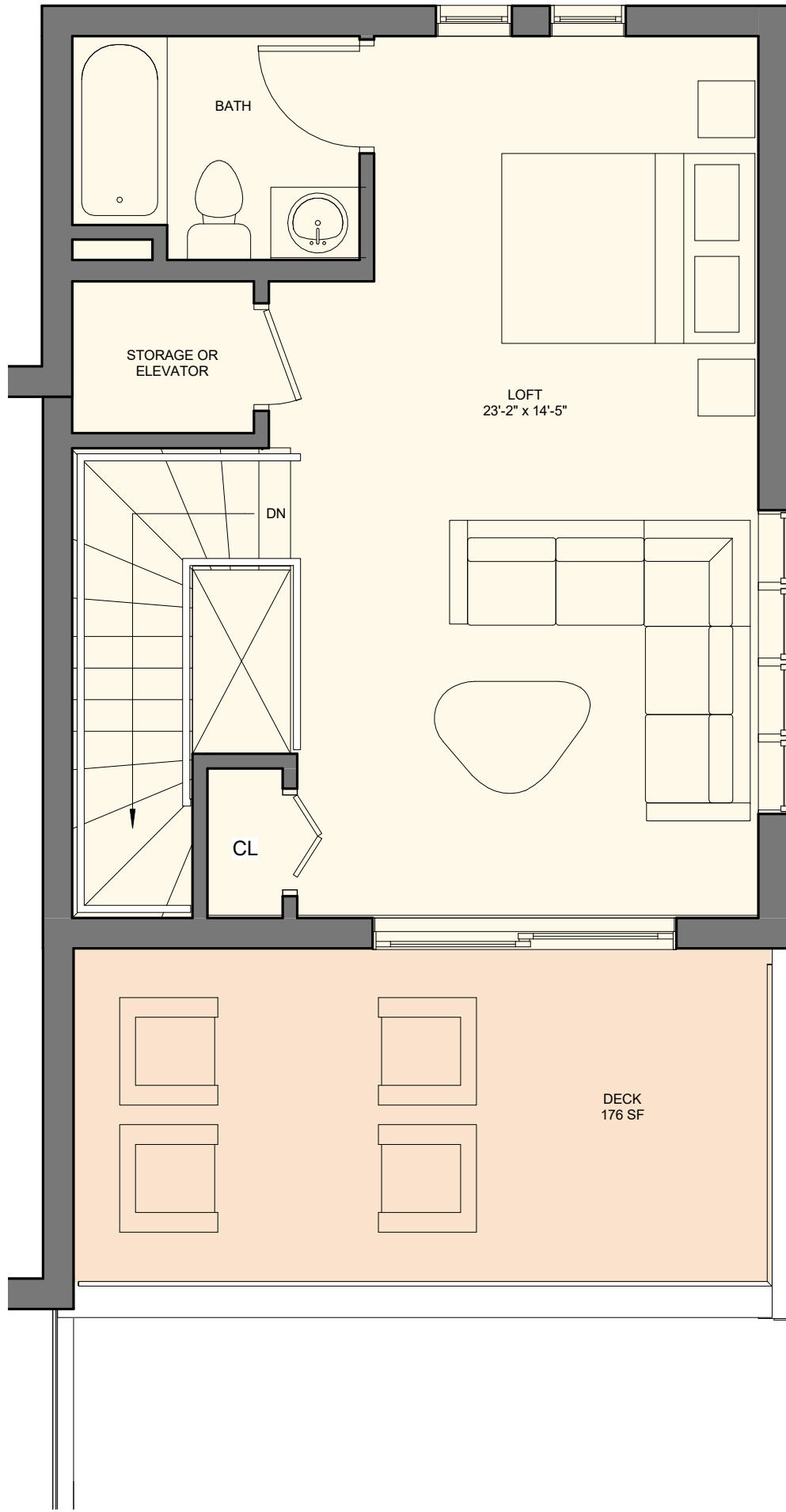
UNIT 1 FOURTH FLOOR PLAN 1/4" = 1'
