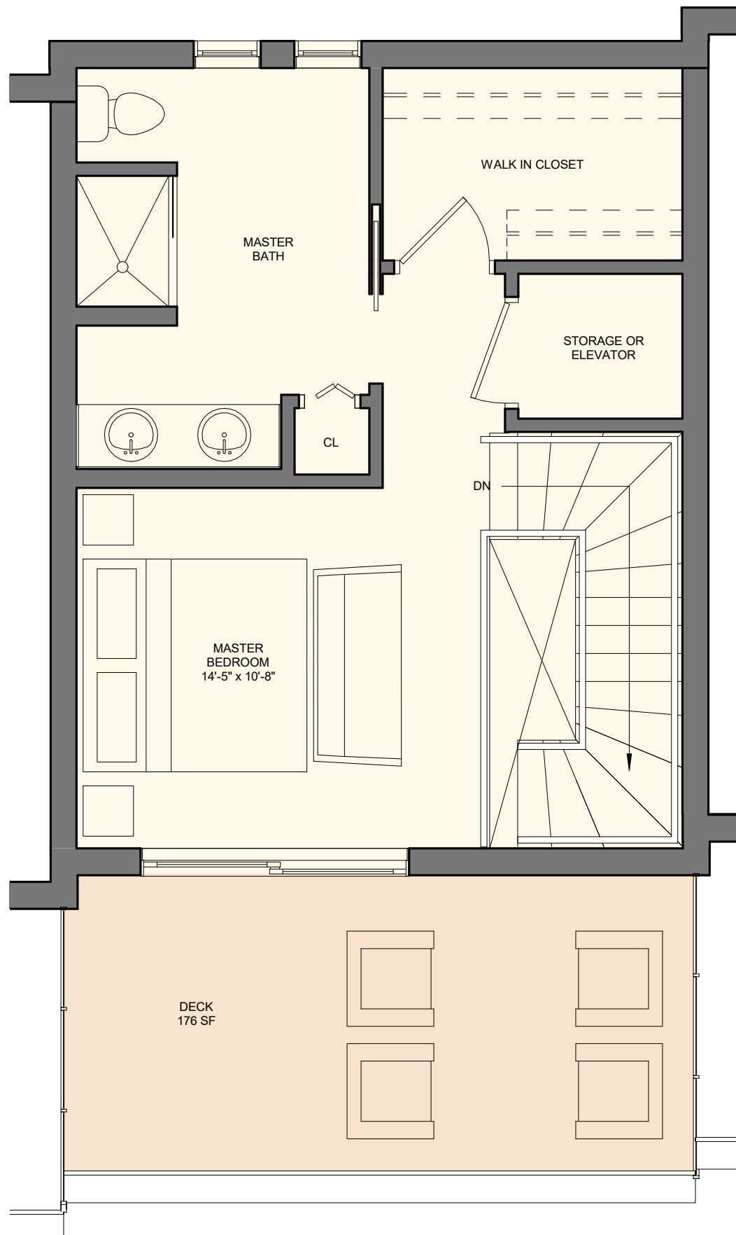
FOURTH FLOOR PLAN OPTION B 1/4" = 1'
