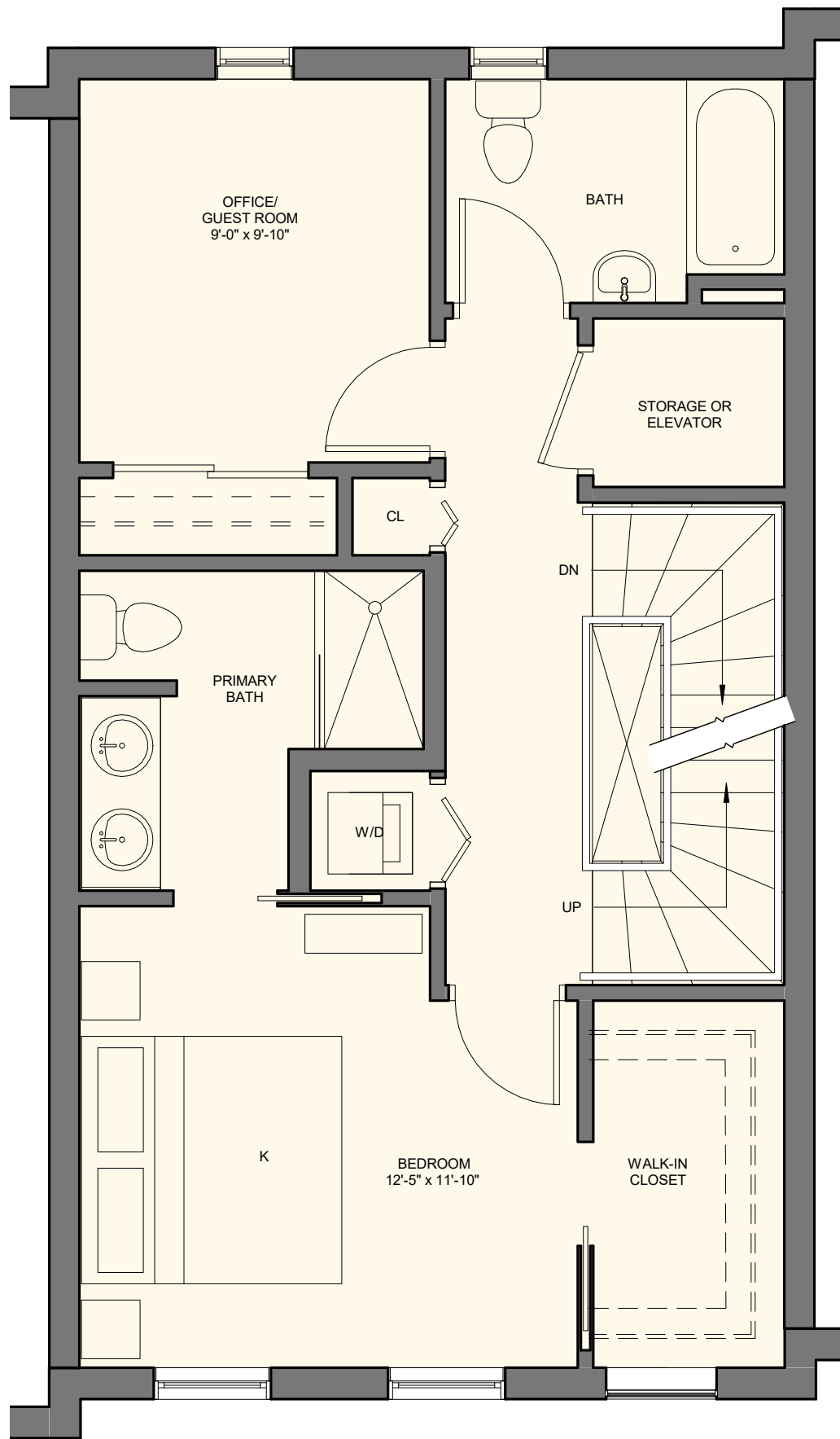
THIRD FLOOR PLAN OPTION B 1/4" = 1'
