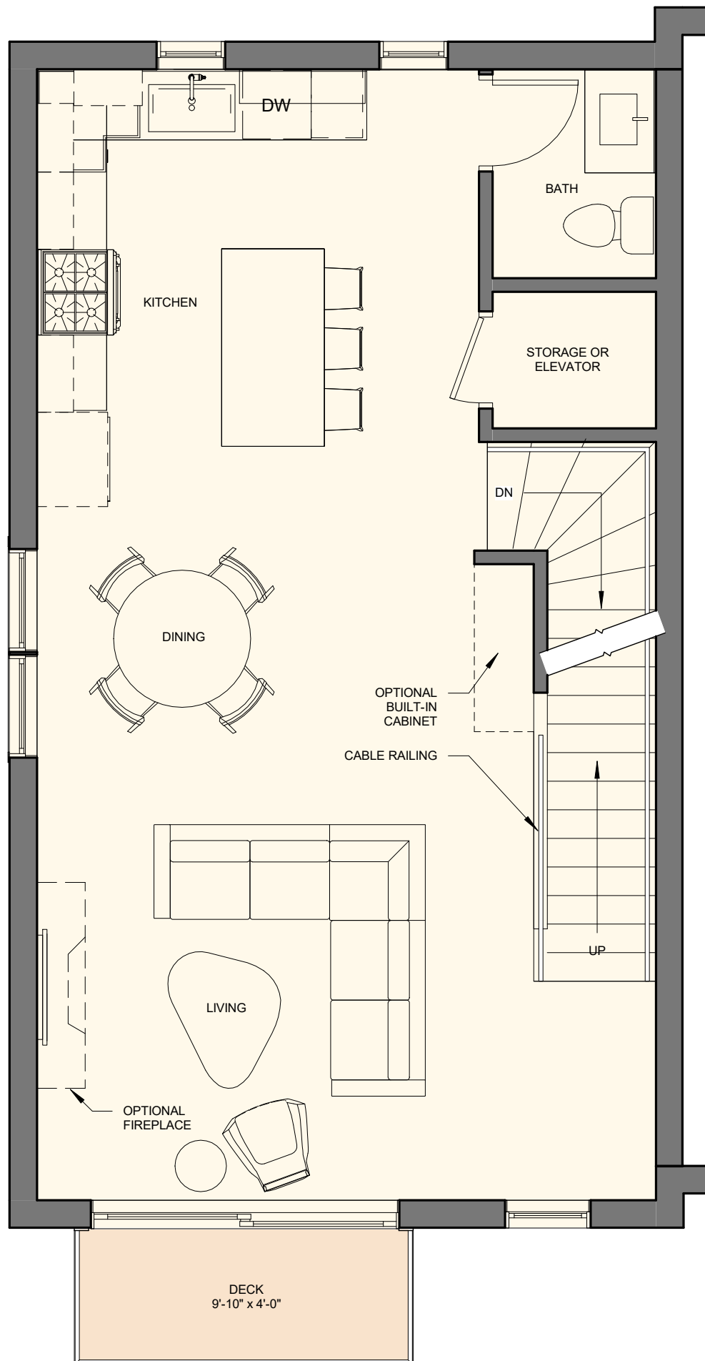
UNIT 7 SECOND FLOOR PLAN 1/4" = 1'
