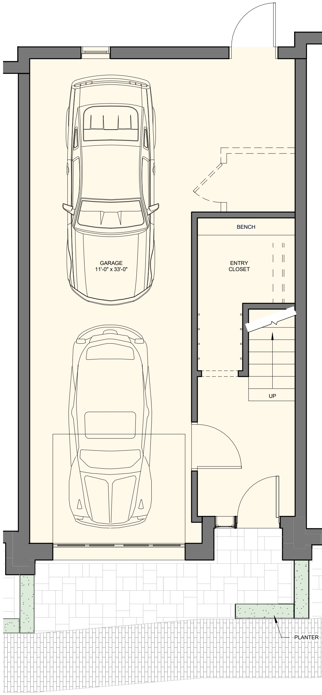
FIRST FLOOR PLAN 1/4" = 1'
